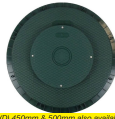
(D) 600mm (24") Flat Cover With Integrated Activated Carbon Filter
