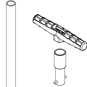
POLYLOK SUPPLIED 18 3/4" x 3/4" PVC PIPE OPTIONAL POLYLOK PRESSURE FILTER WRENCH KIT PART NO. 3014-PFW
