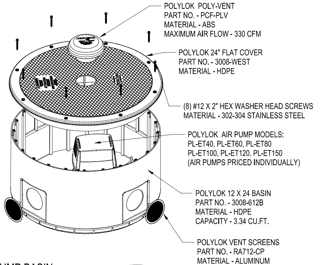
POLYLOK AIR PUMP BASIN PART NO. 3008-APB
